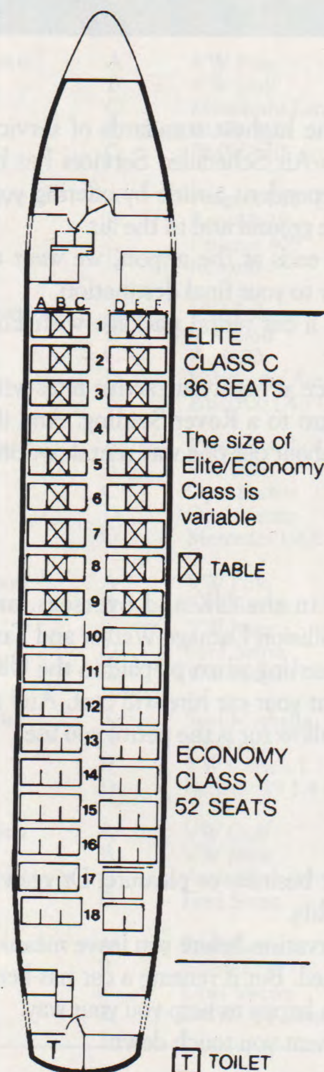
BAe 146 SERIES 300
