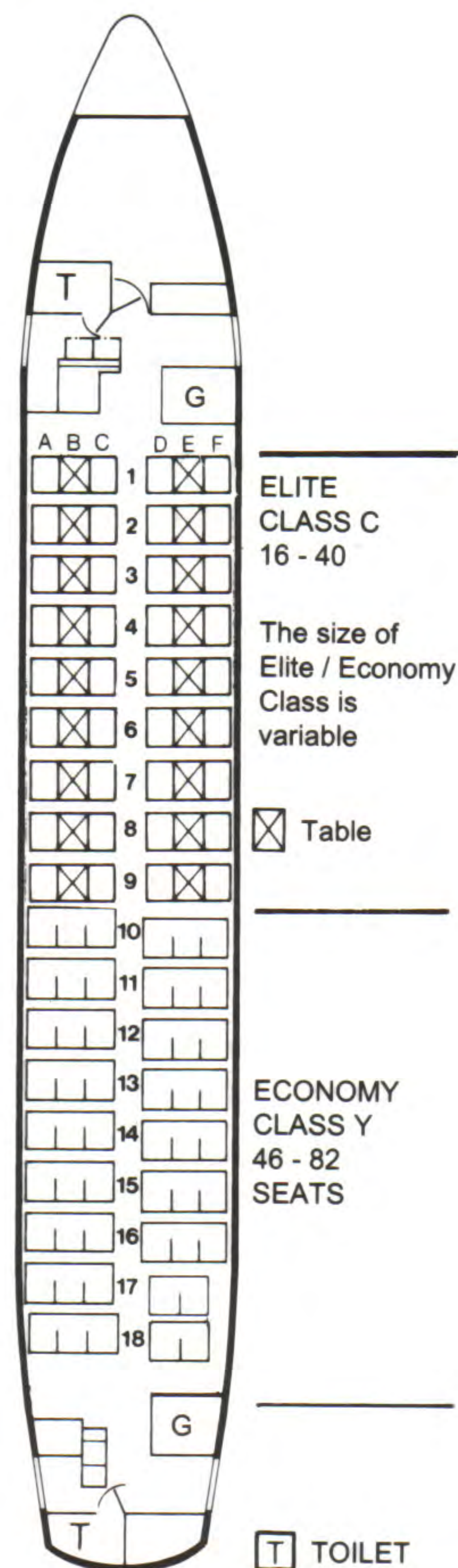
BAe 146 SERIES 300
