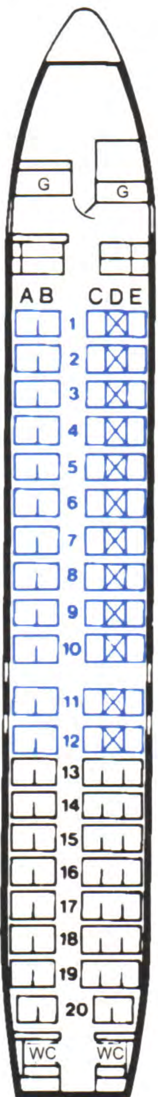
BAe 1-11 SERIES 500
