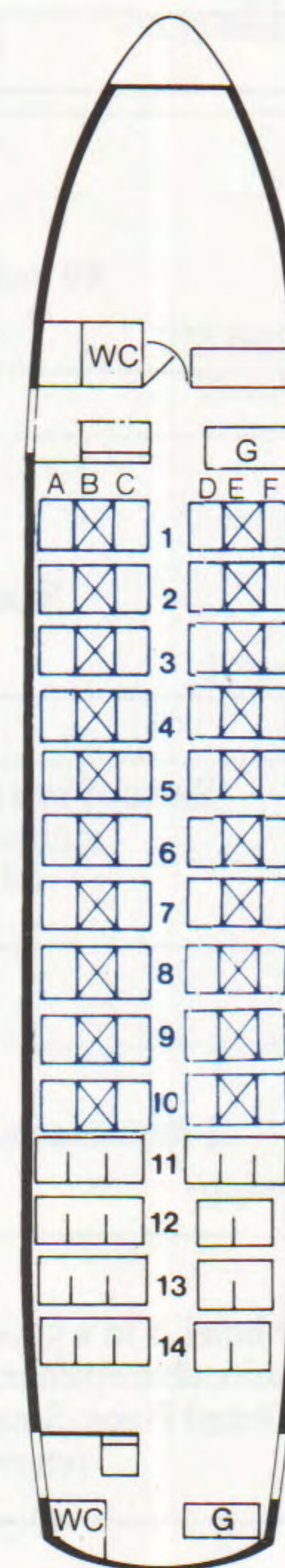
BAe 146 SERIES 100
