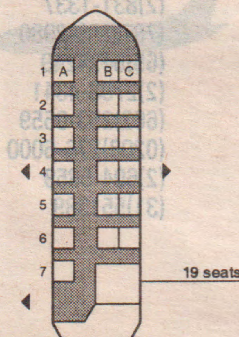
Jetstream 31
